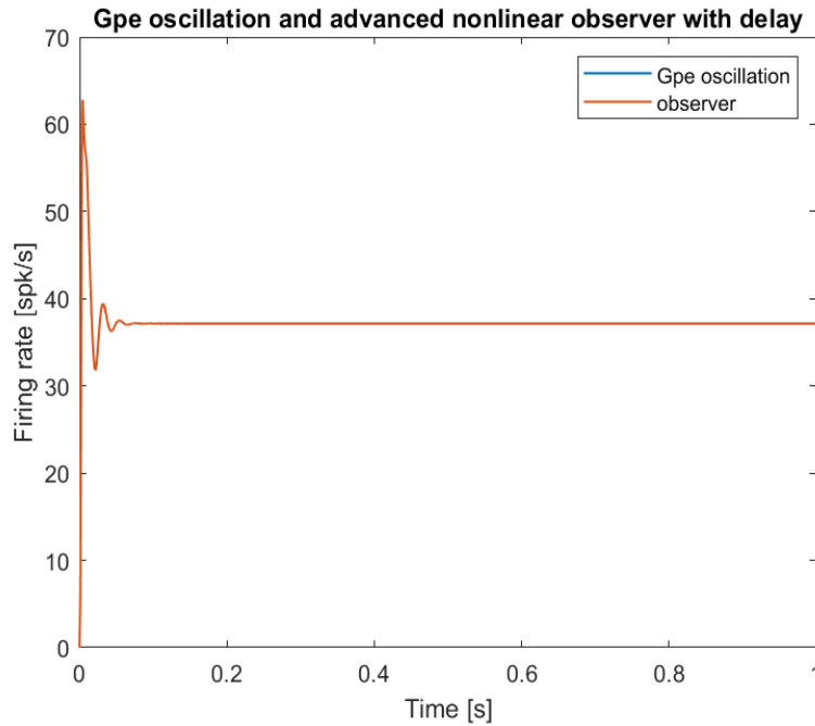
Figure12. Gpe oscillation and advanced nonlinear observer with delay
