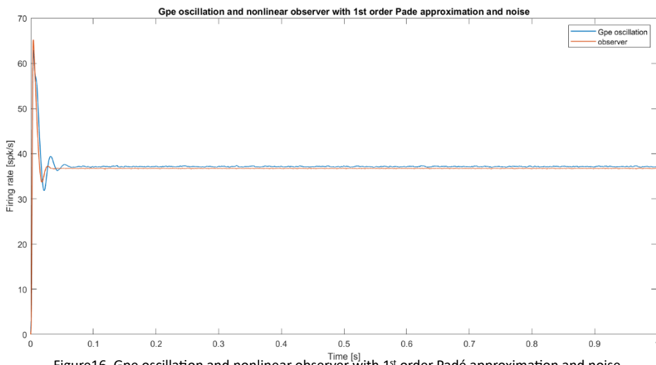
Figure16. Gpe oscillation and nonlinear observer with 1 st order Padé approximation and noise
