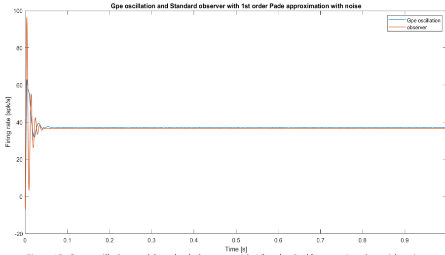
Figure15. Gpe oscillation and Standard observer with 1 st order Padé approximation with noise
