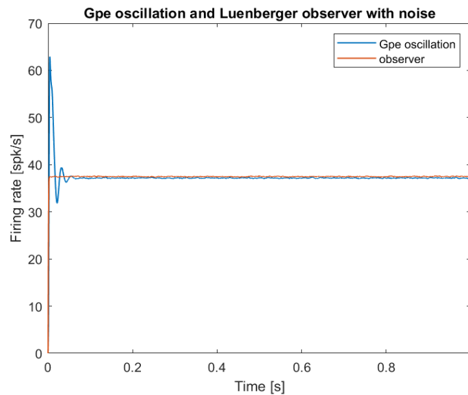
Figure14. Gpe oscillation and Luenberger observer with noise
