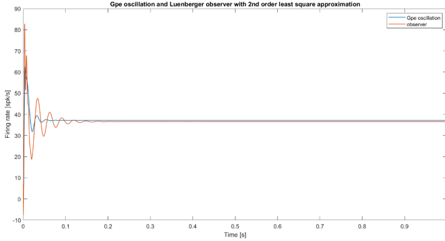
Figure8. Gpe oscillation and Luenberger observer with 2 nd order least square approximation
