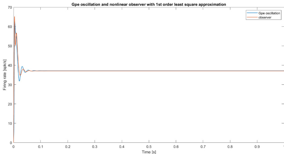
Figure11. Gpe oscillation and nonlinear observer with 1 st square approximation
