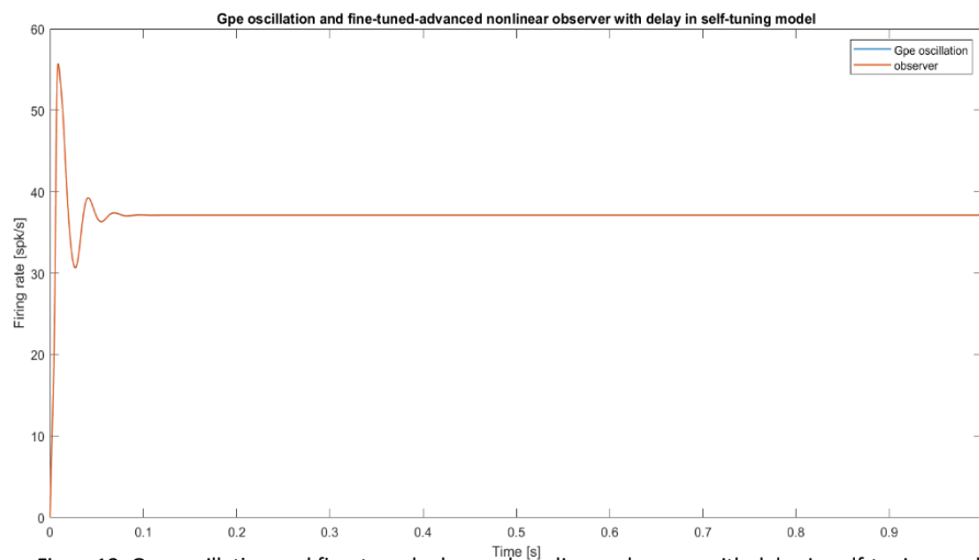
Figure13. GPe oscillation and fine-tuned advanced nonlinear observer with delay in self-tuning model
