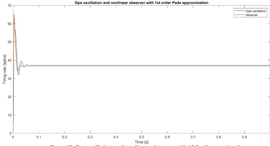
Figure10. Gpe oscillation and nonlinear observer with 1 st Padé approximation
