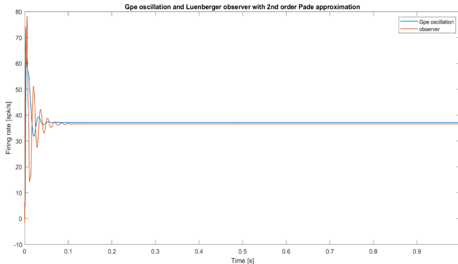
Figure6. Gpe oscillation and Luenberger observer with 2 nd order Padé approximation
