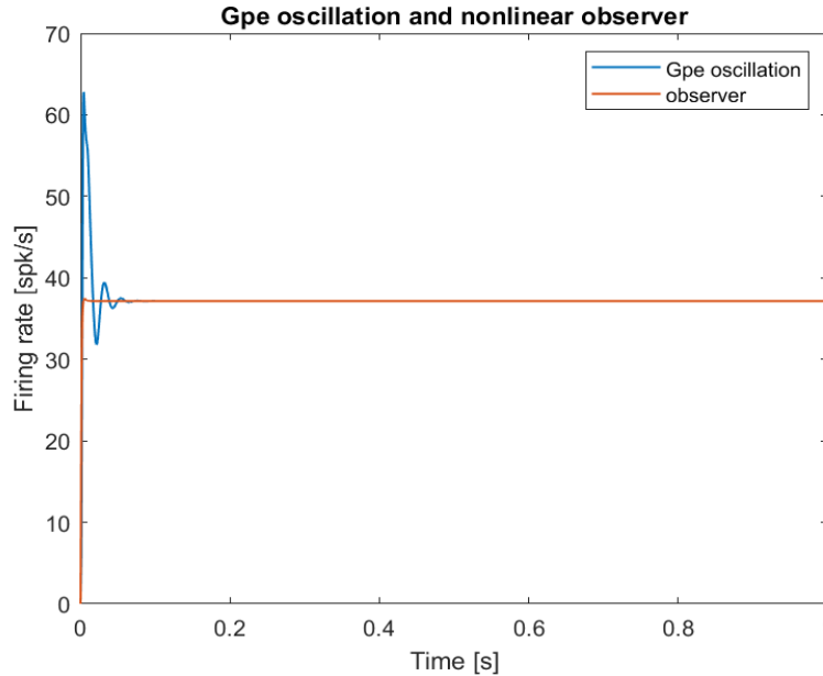
Figure9. Gpe oscillation and nonlinear observer
