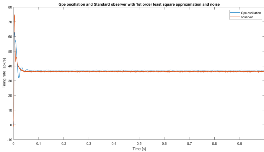
Figure17. Gpe oscillation and standard observer with 1 st order least square approximation and noise
